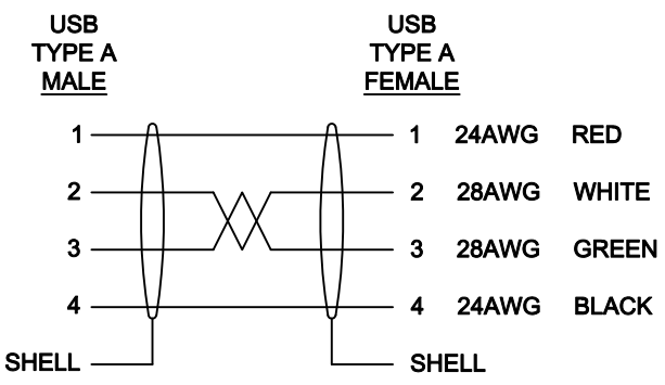
MALE-TO-FEMALE PINOUT
