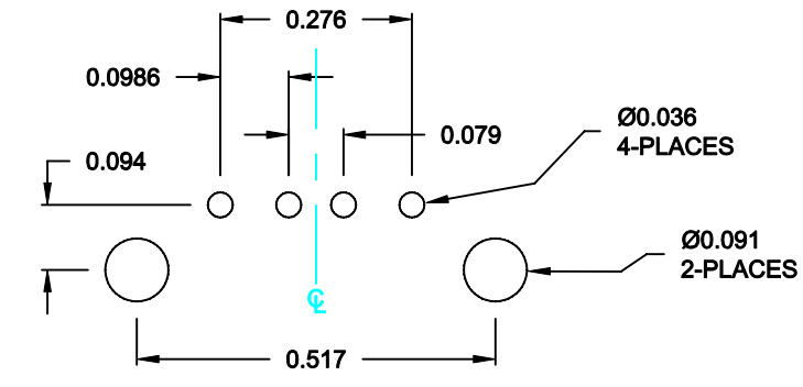
RECOMMENDED PCB LAYOUT SCALE = 3 : 1
