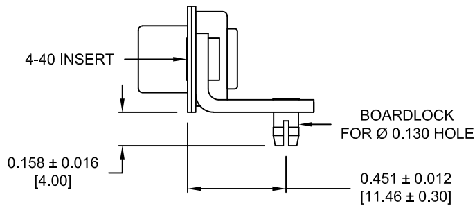
MOUNTING HARDWARE
