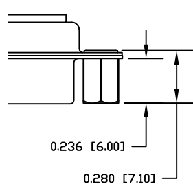
3 ..... 0.236" MATING SIDE
