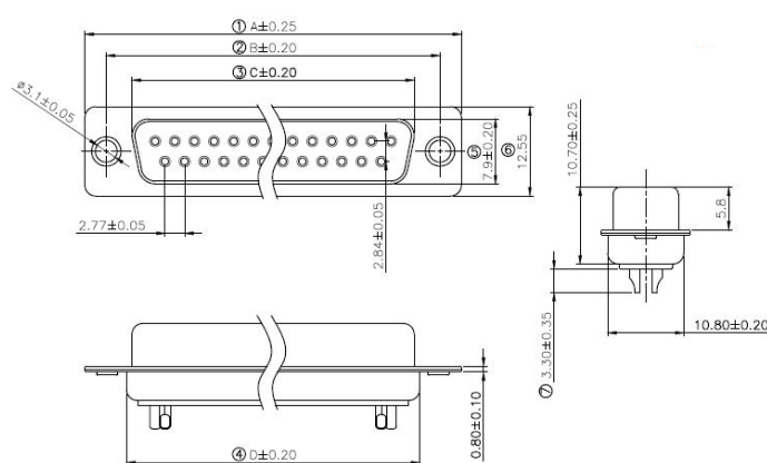
Male Dimensions
