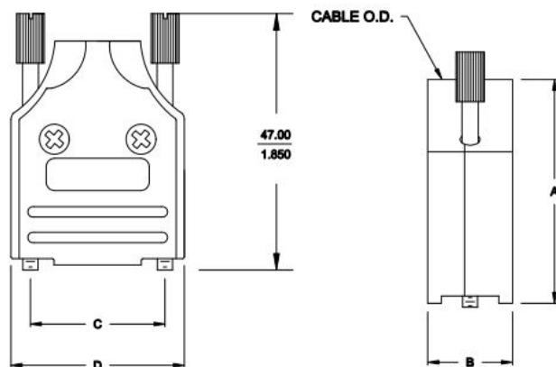
Hood Dimensions
