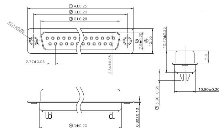
Female Dimensions
