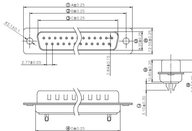
Male Dimensions
