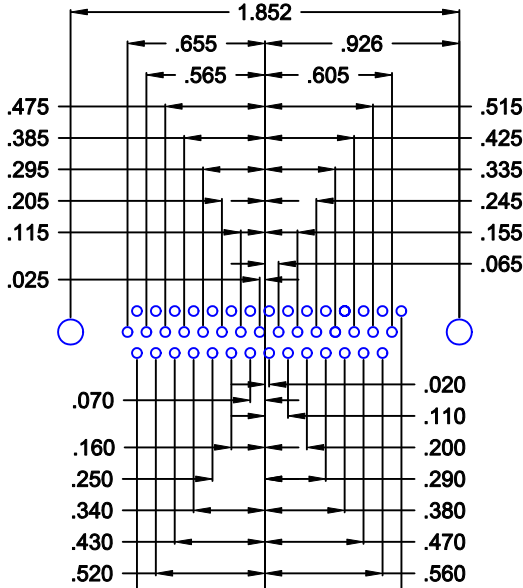
44 POSITION
