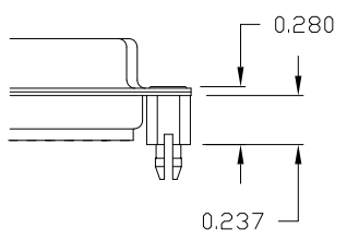
90 ..... 0.237" (BOARD SIDE)
