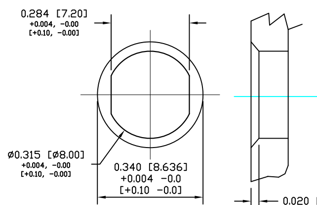
PANEL CUTOUT
