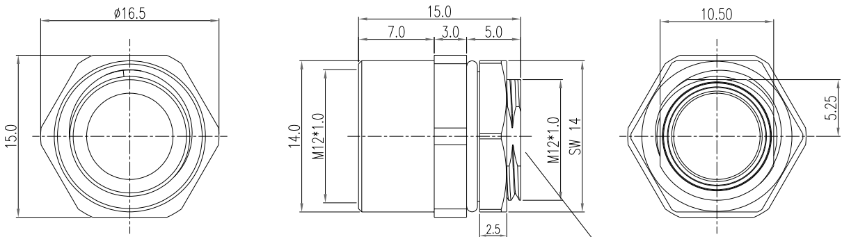
SHELL+O-RING A+NUT
