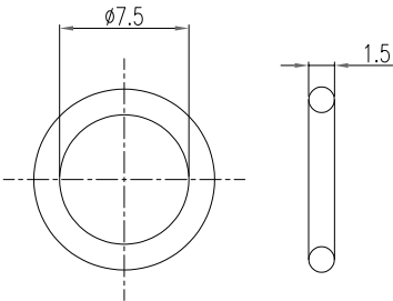
O-RING B
