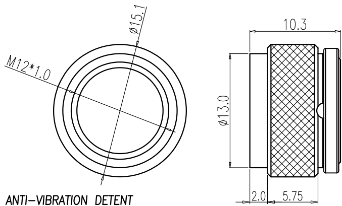
NUT & ANTI-VIBRATION DETENT
