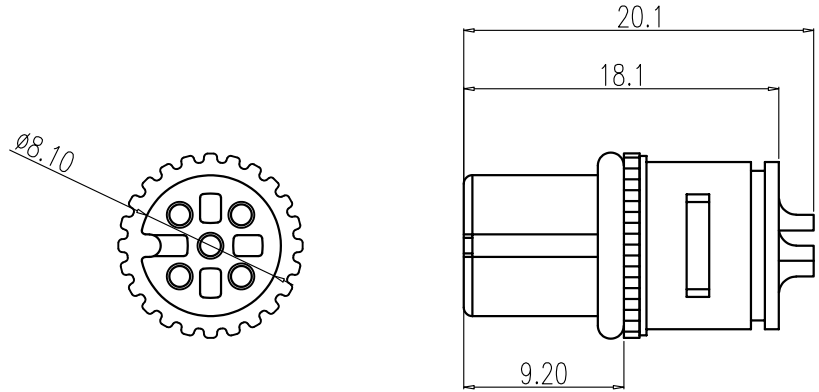
HOUSING & O-RING & SHELL
